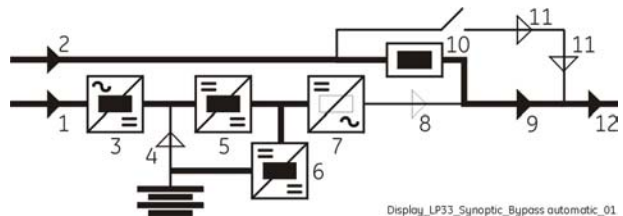
Display_LP33_Synoptic_Bypass automatic_01
