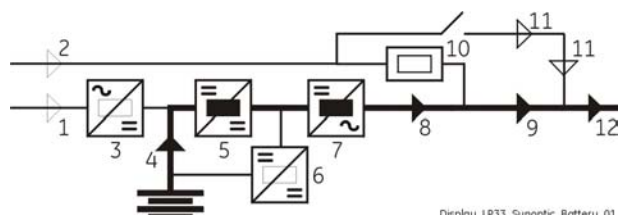
Display_LP33_Synoptic_Battery_01
